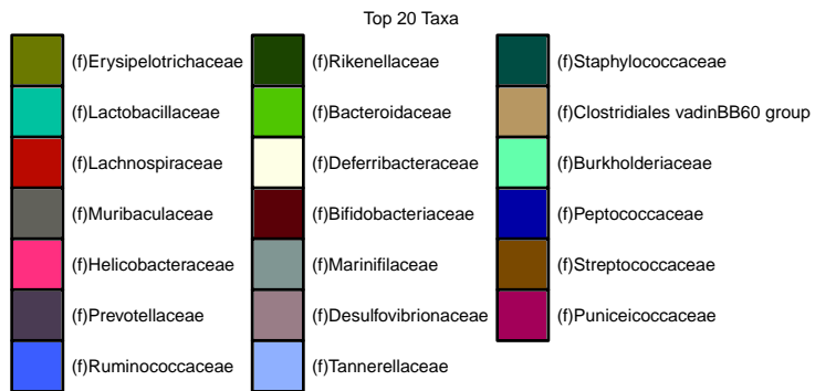
Figure 28: Family level abundances-UNFILTERED
