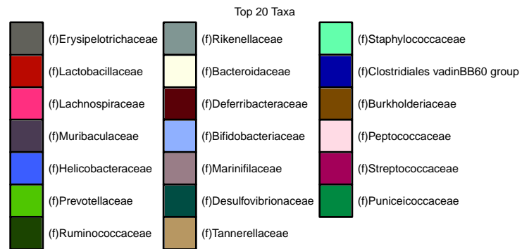
Figure 30: Family level abundances-FILTERED & RESCALED
