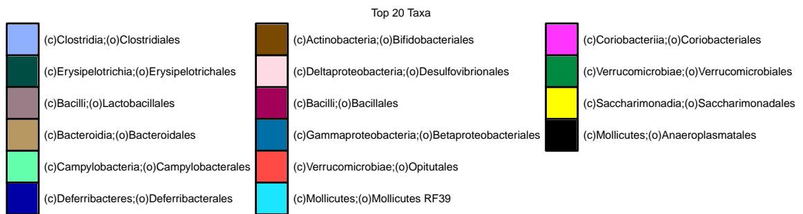
Figure 27: Order level abundances-FILTERED & RESCALED
