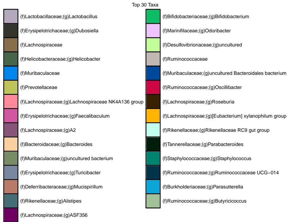
Figure 32: Genus level abundances-FILTERED: 15 genus level taxa removed
