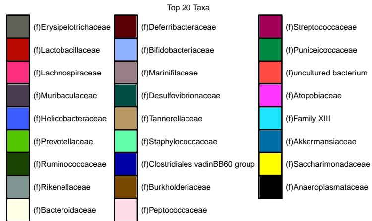
Figure 29: Family level abundances-FILTERED: 2 family level taxa removed
