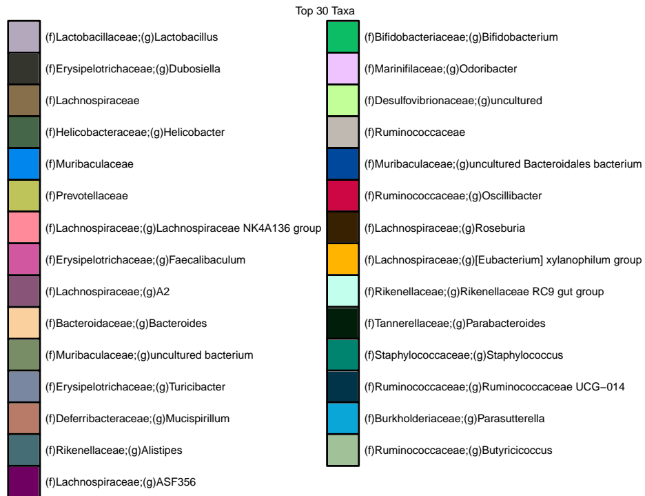
Figure 33: Genus level abundances-FILTERED & RESCALED
