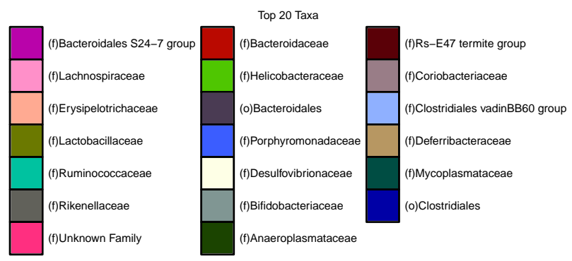
Figure 30: Family level abundances-FILTERED & RESCALED 26
