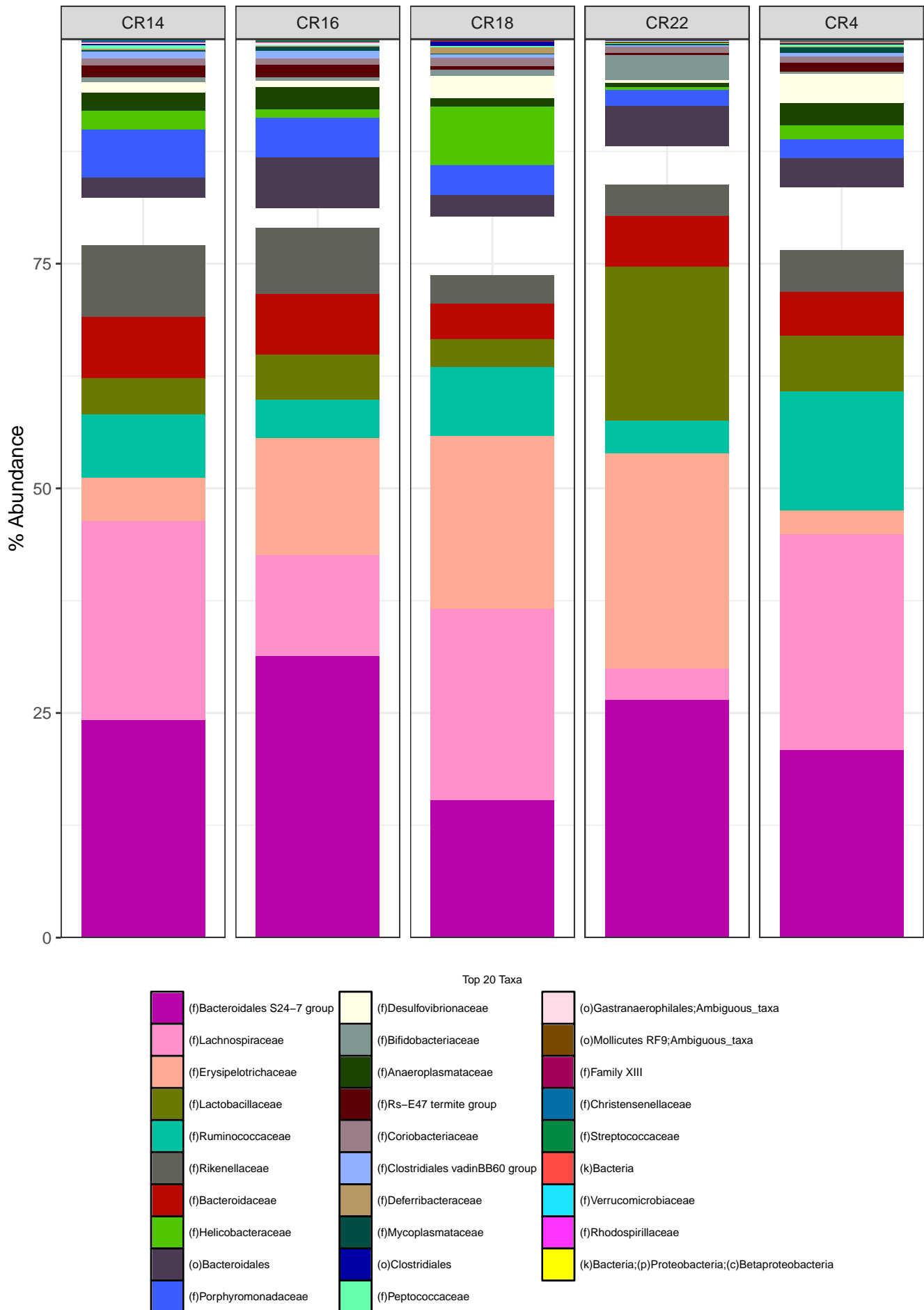
Figure 29: Family level abundances-FILTERED: 2 family level taxa removed
