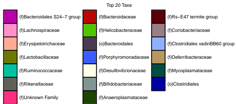
Figure 28: Family level abundances-UNFILTERED
