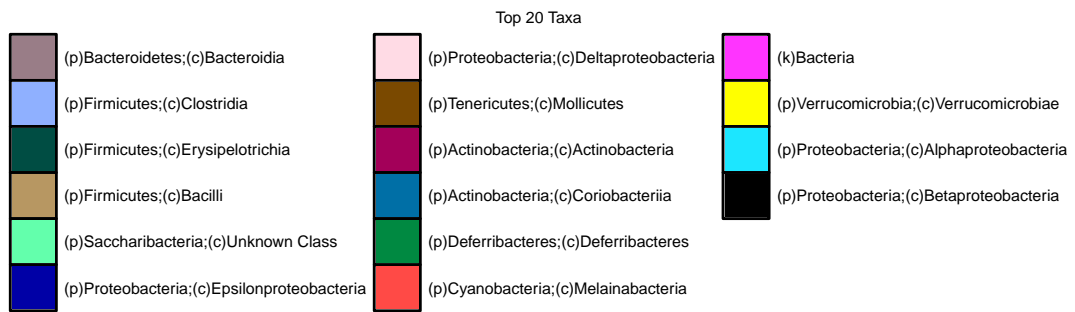
Figure 23: Class level abundances-FILTERED: 0 class level taxa removed
