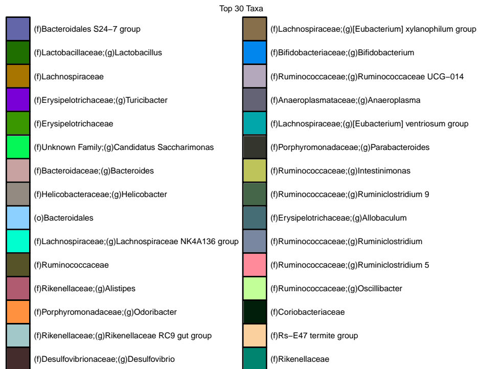
Figure 32: Genus level abundances-FILTERED: 15 genus level taxa removed
