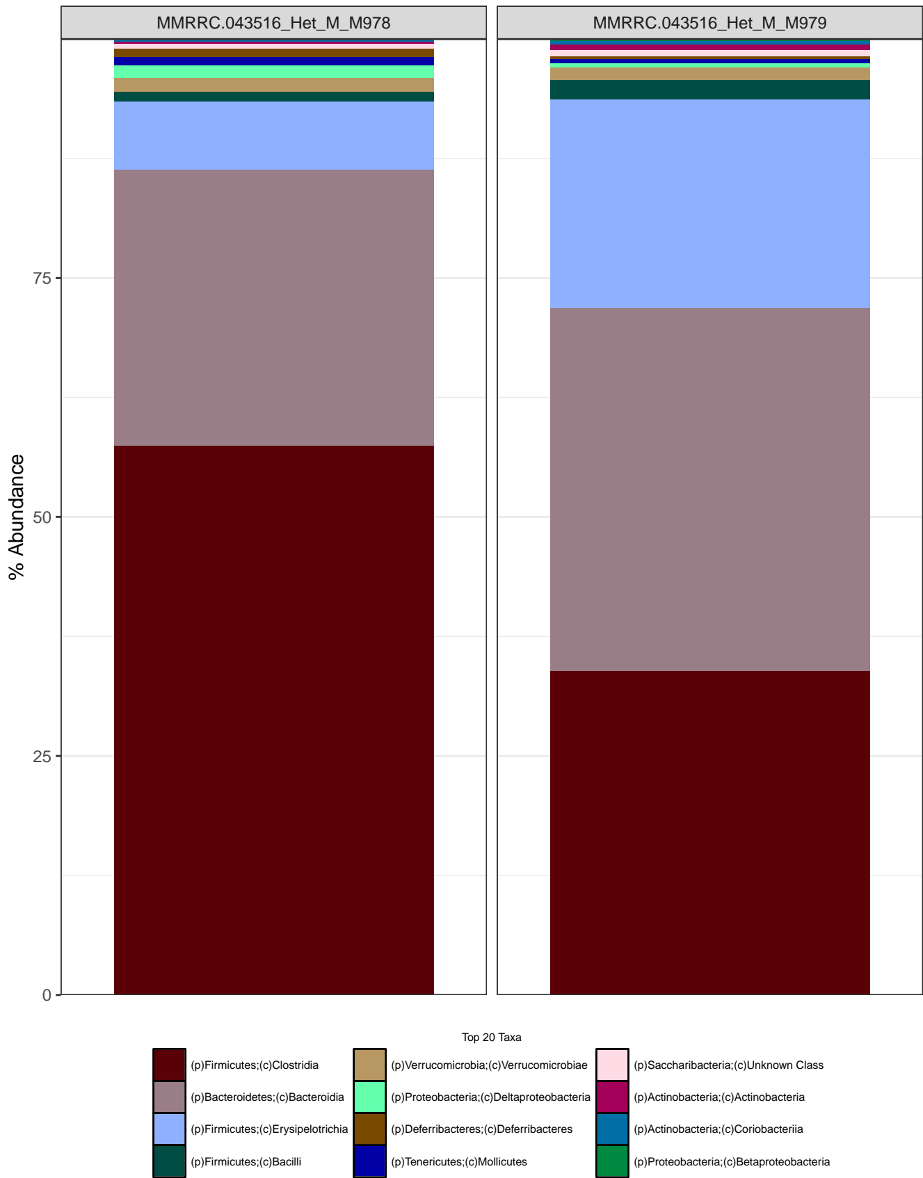
Figure 23: Class level abundances-FILTERED: 5 class level taxa removed
