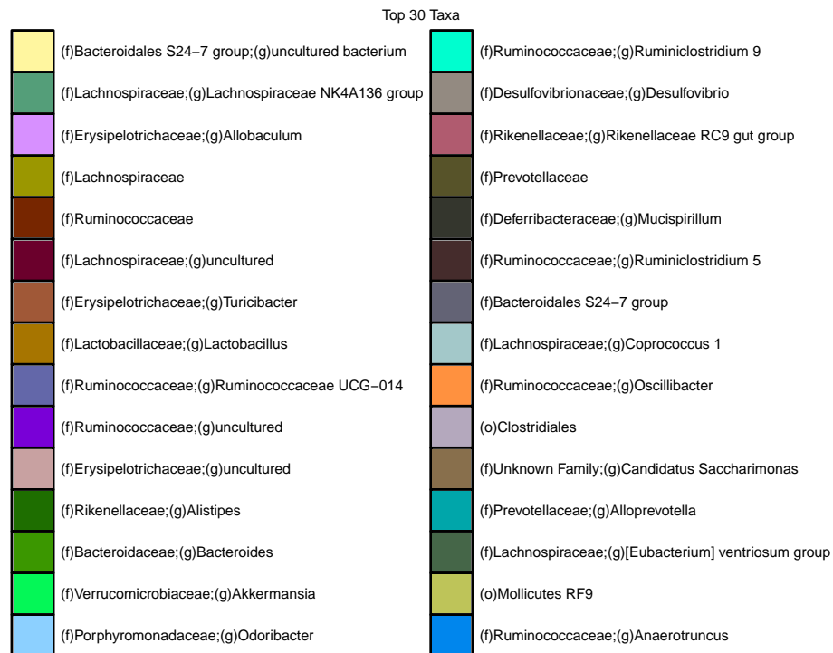
Figure 32: Genus level abundances-FILTERED: 21 genus level taxa removed
