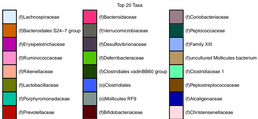
Figure 29: Family level abundances-FILTERED: 9 family level taxa removed
