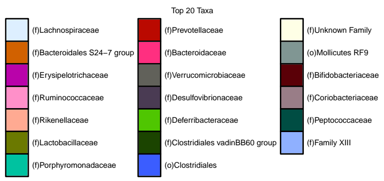
Figure 28: Family level abundances-UNFILTERED 24
