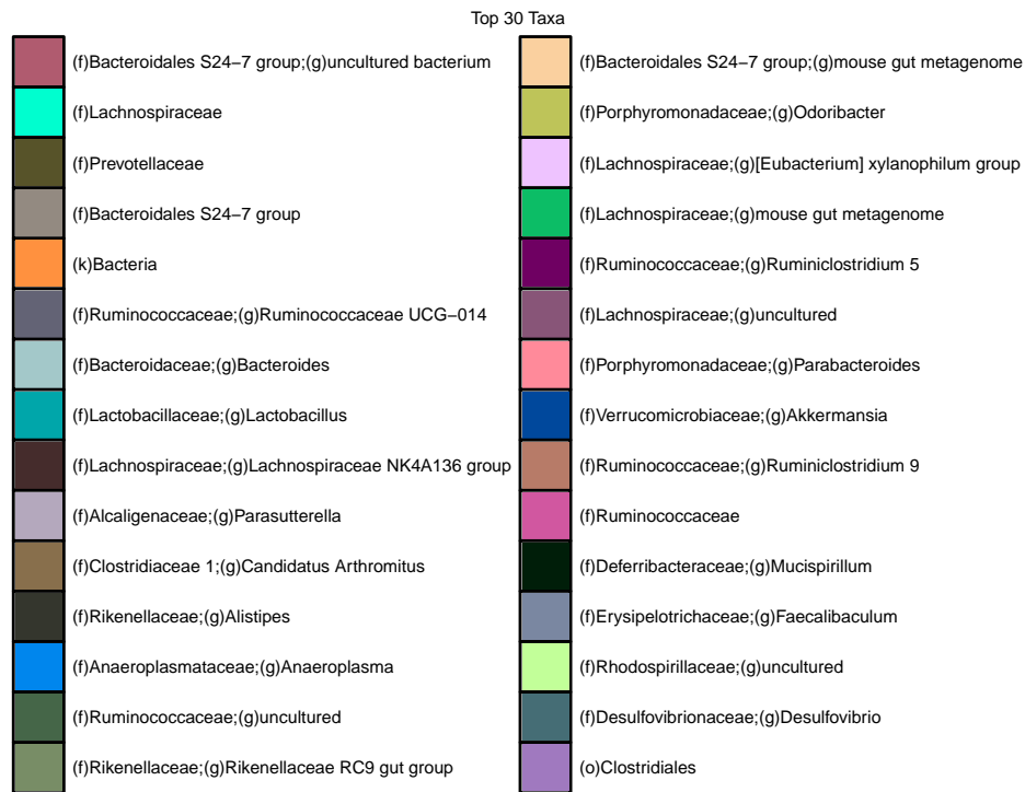
Figure 32: Genus level abundances-FILTERED: 12 genus level taxa removed
