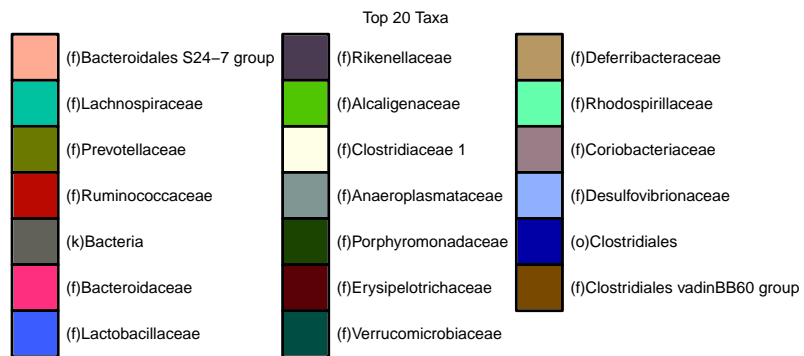
Figure 30: Family level abundances-FILTERED & RESCALED
