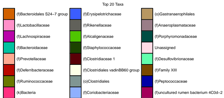
Figure 29: Family level abundances-FILTERED: 8 family level taxa removed
