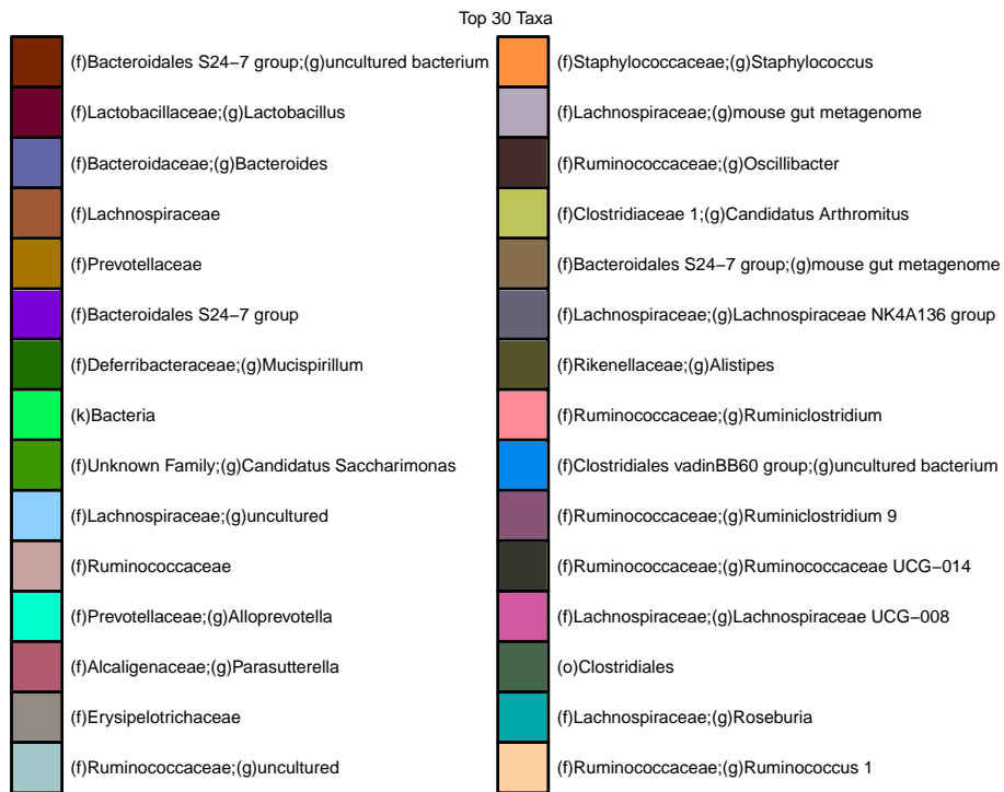
Figure 32: Genus level abundances-FILTERED: 19 genus level taxa removed
