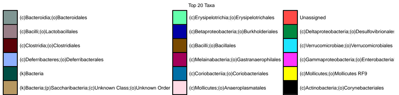
Figure 25: Order level abundances-UNFILTERED
