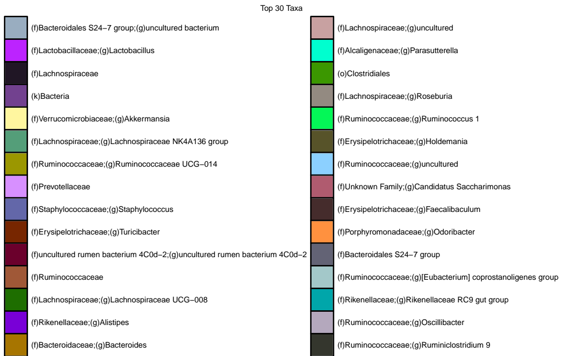
Figure 32: Genus level abundances-FILTERED: 22 genus level taxa removed
