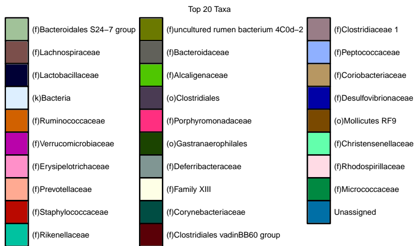
Figure 29: Family level abundances-FILTERED: 7 family level taxa removed
