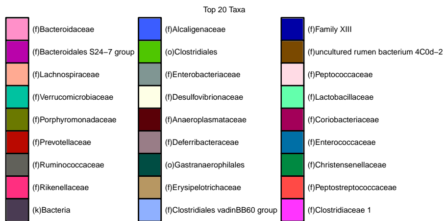
Figure 29: Family level abundances-FILTERED: 4 family level taxa removed
