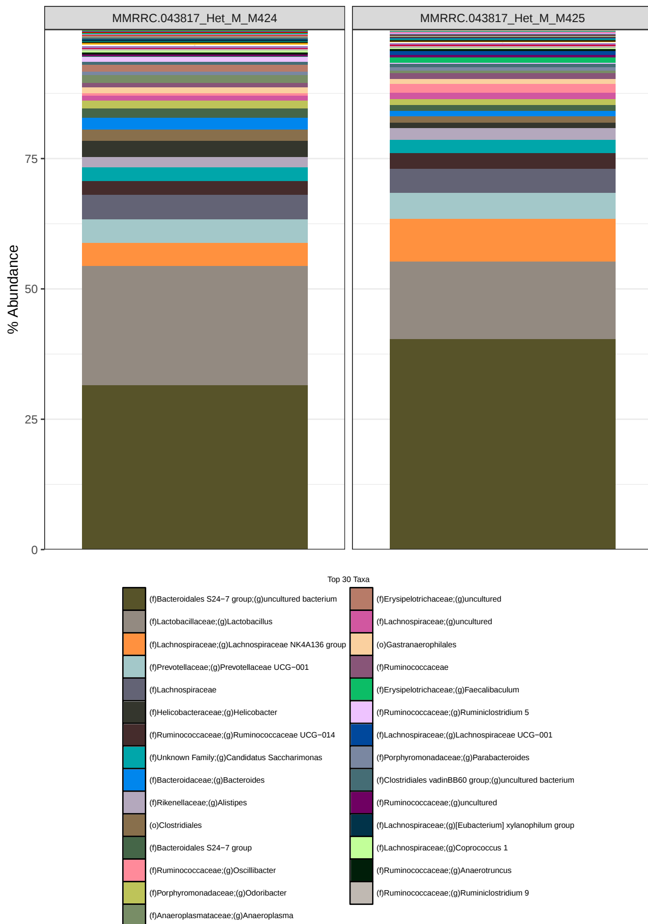
Figure 32: Genus level abundances-FILTERED: 17 genus level taxa removed
