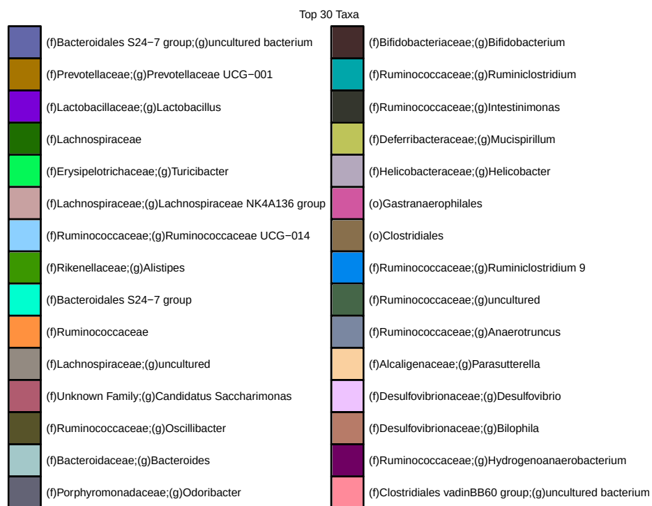
Figure 31: Genus level abundances-UNFILTERED
