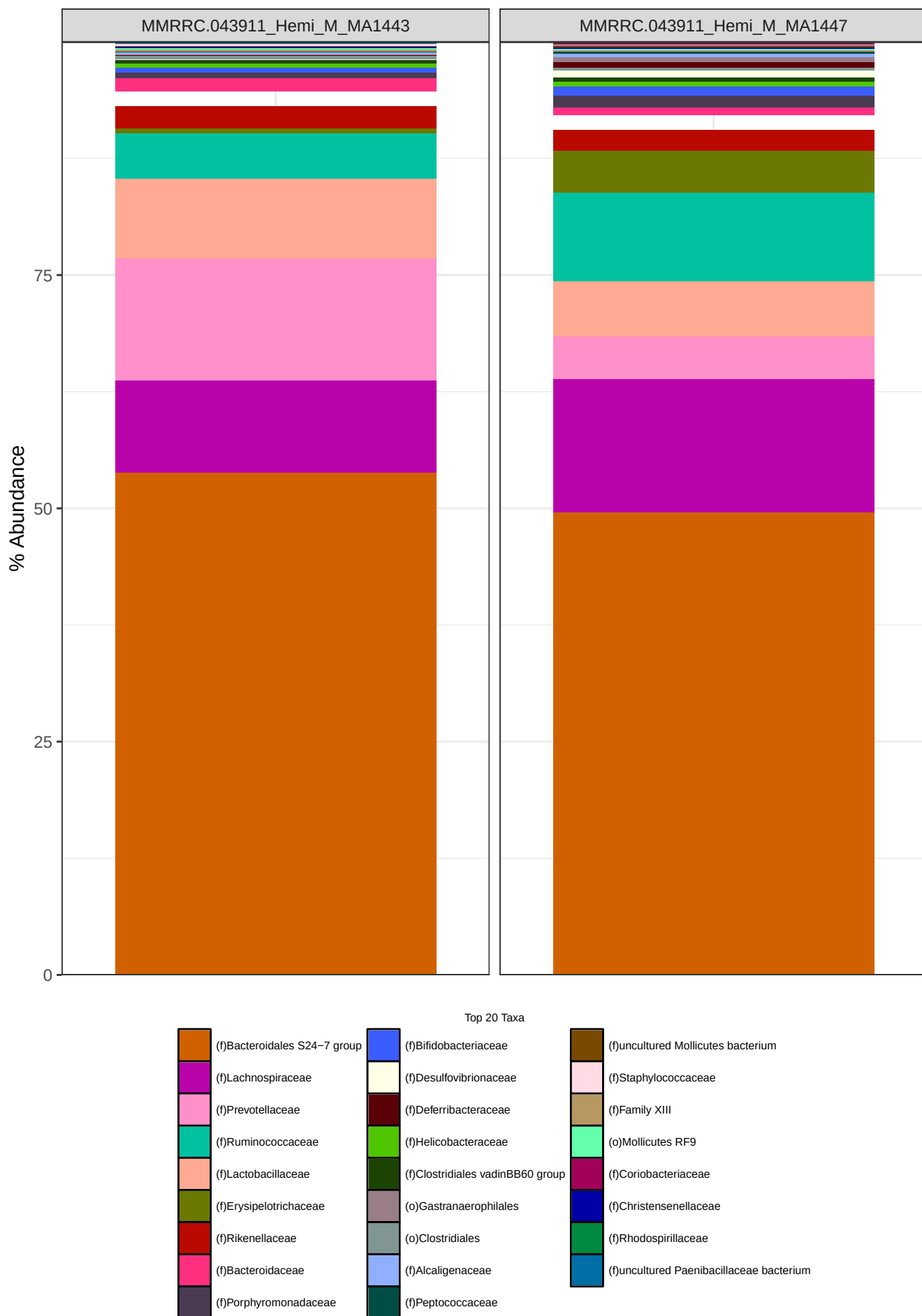
Figure 29: Family level abundances-FILTERED: 6 family level taxa removed
