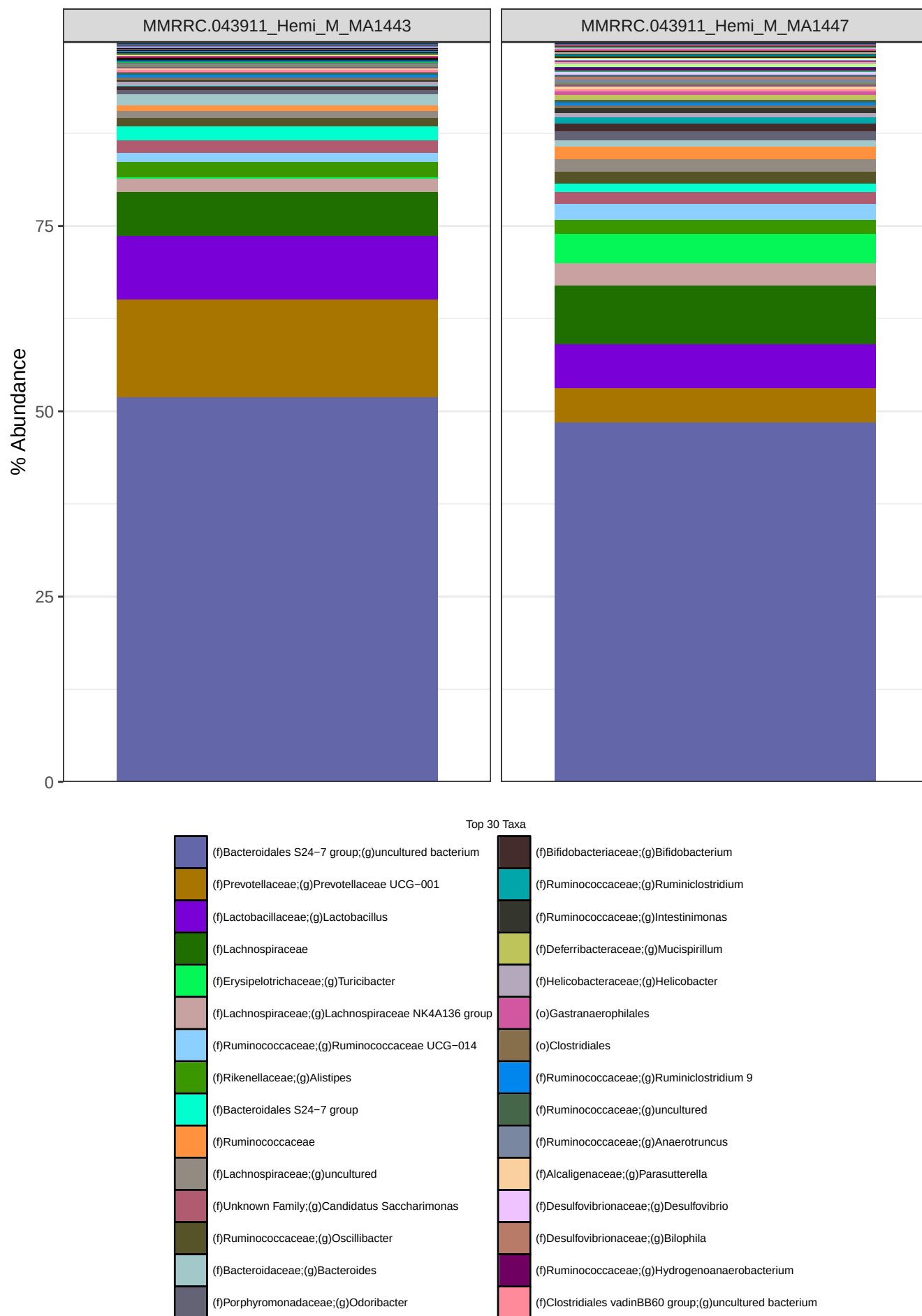
Figure 32: Genus level abundances-FILTERED: 15 genus level taxa removed
