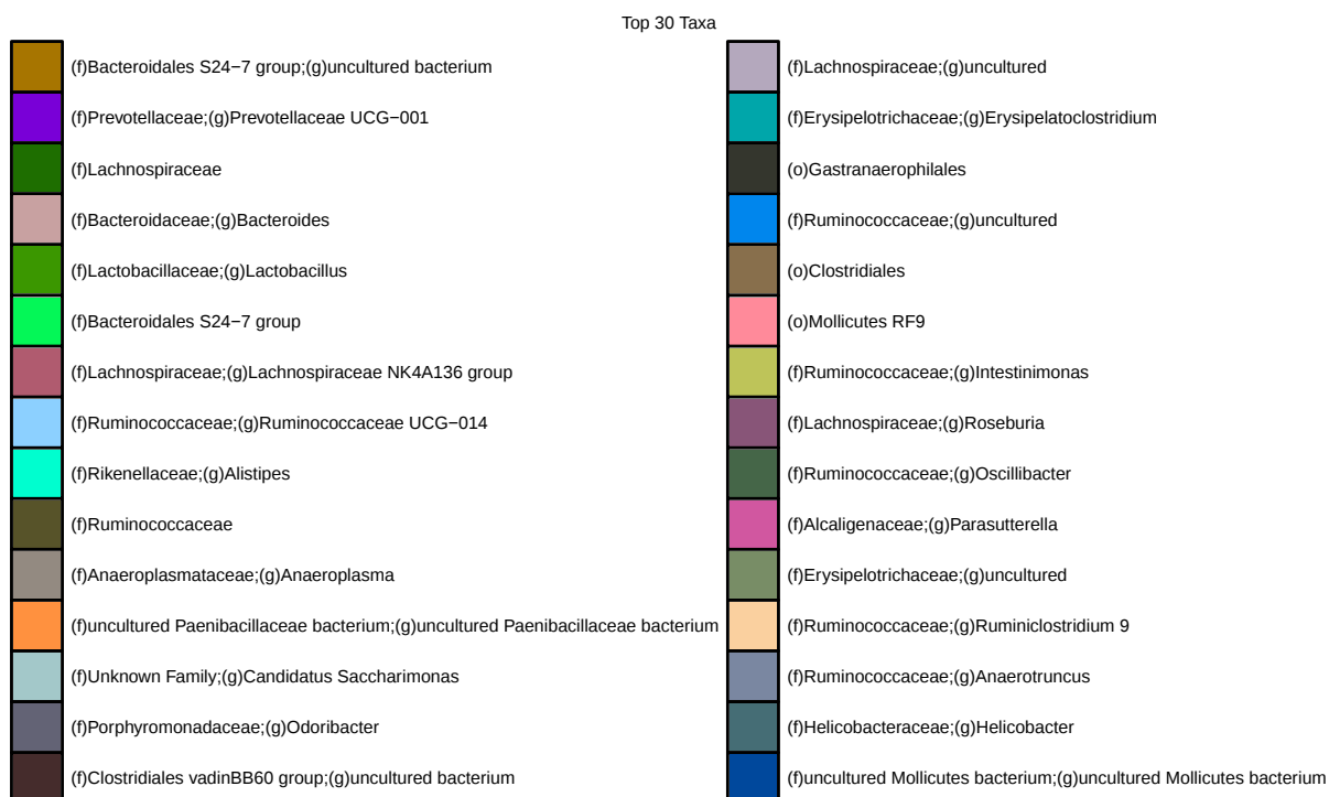
Figure 32: Genus level abundances-FILTERED: 26 genus level taxa removed
