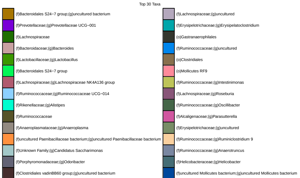
Figure 33: Genus level abundances-FILTERED & RESCALED
