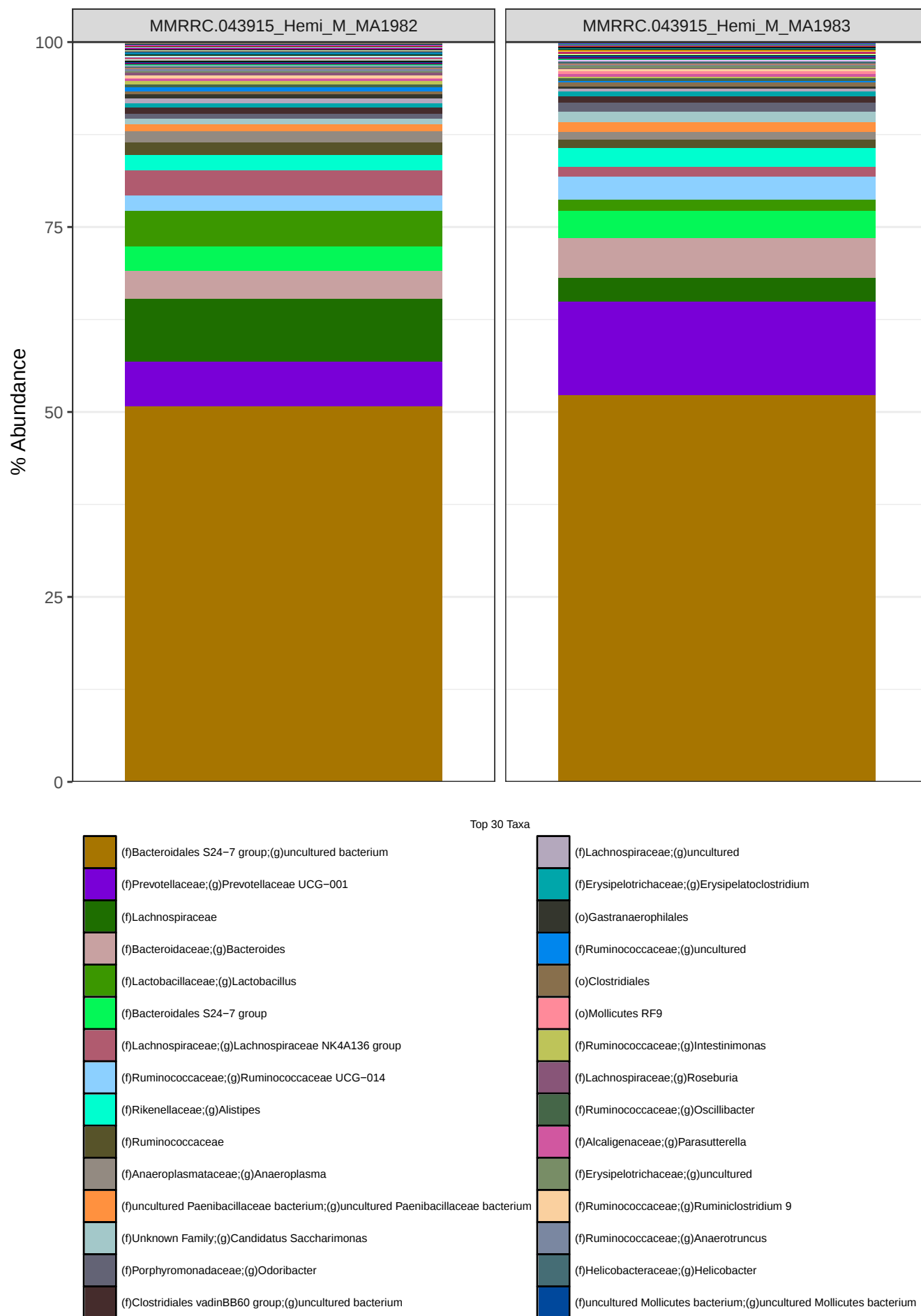
Figure 31: Genus level abundances-UNFILTERED
