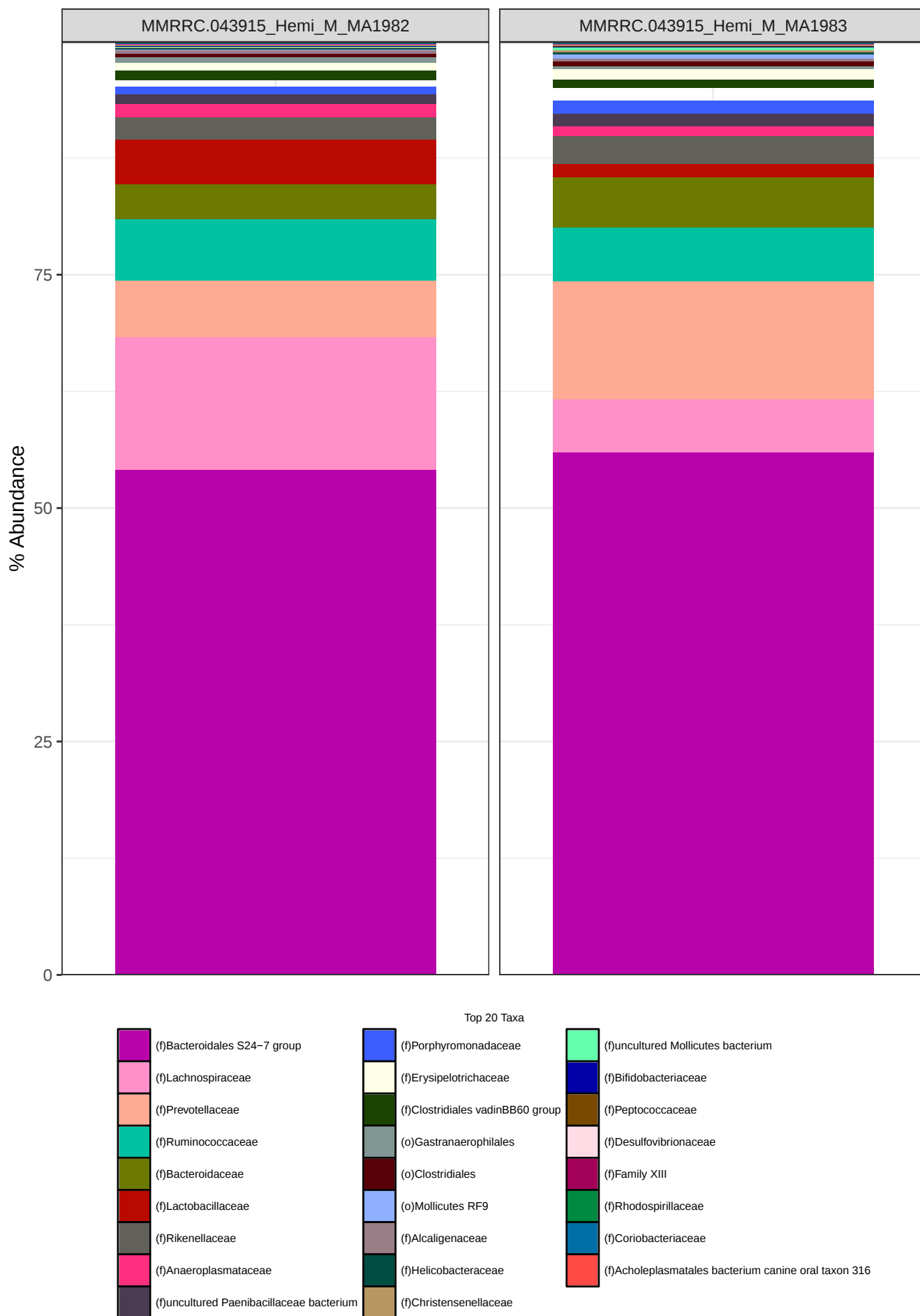
Figure 29: Family level abundances-FILTERED: 5 family level taxa removed
