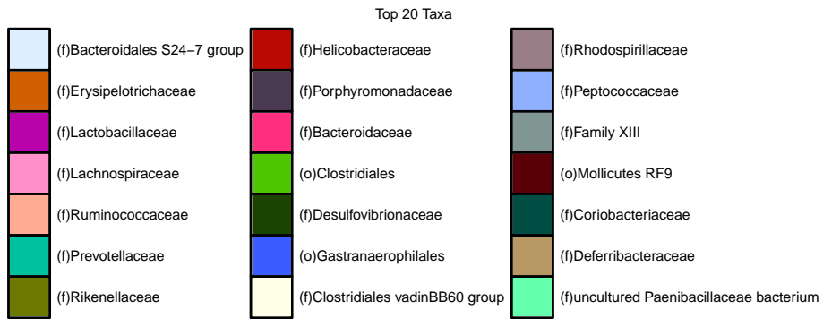
Figure 29: Family level abundances-FILTERED: 12 family level taxa removed
