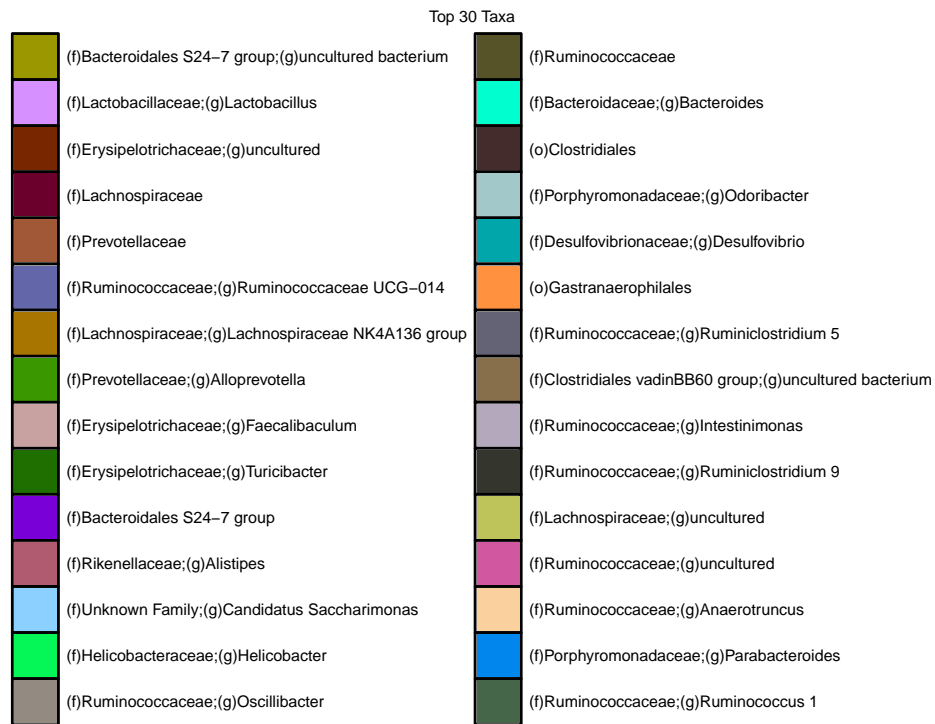
Figure 32: Genus level abundances-FILTERED: 29 genus level taxa removed
