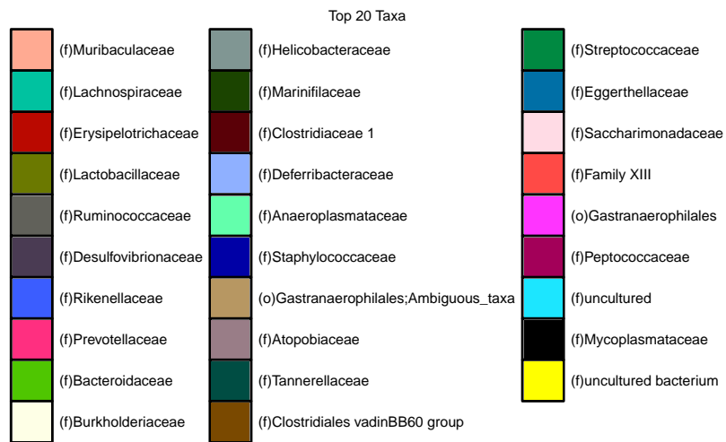
Figure 29: Family level abundances-FILTERED: 3 family level taxa removed
