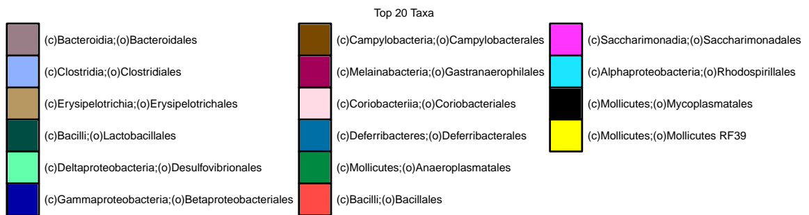
Figure 26: Order level abundances-FILTERED: 1 order level taxa removed
