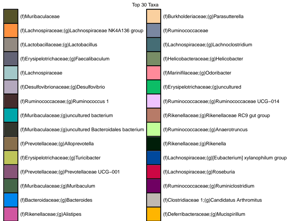
Figure 32: Genus level abundances-FILTERED: 12 genus level taxa removed
