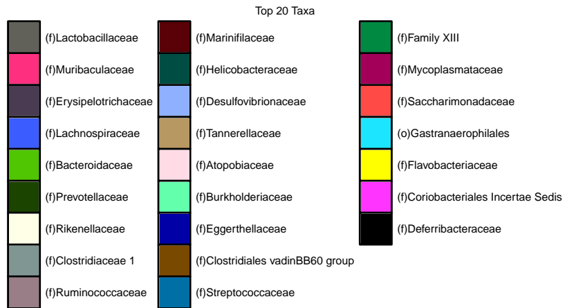
Figure 29: Family level abundances-FILTERED: 4 family level taxa removed
