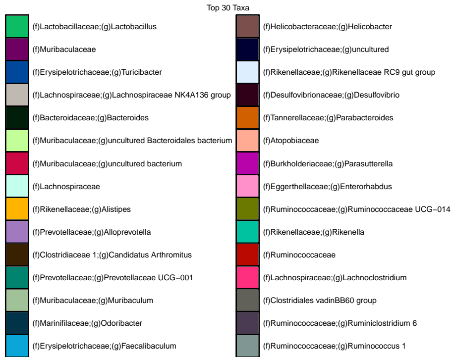
Figure 32: Genus level abundances-FILTERED: 14 genus level taxa removed
