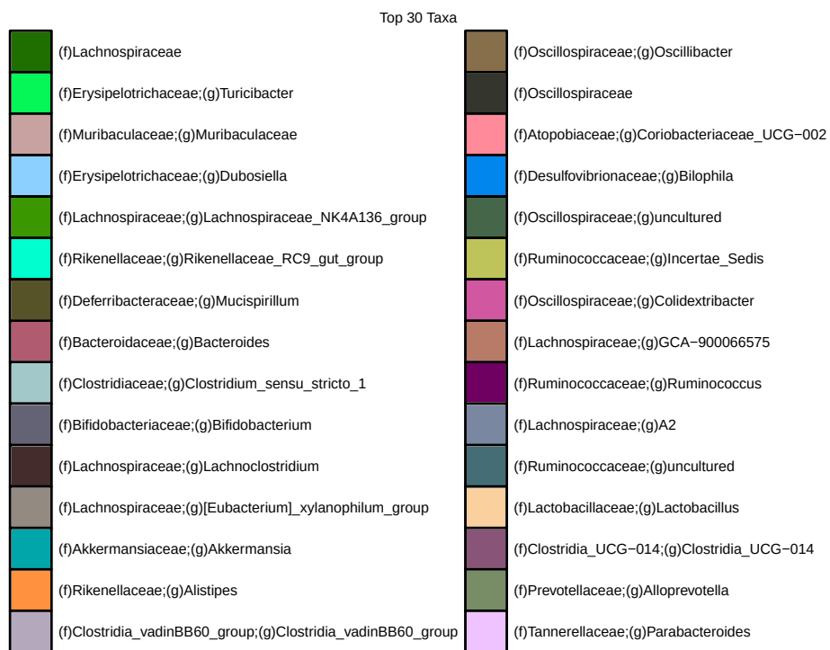
Figure 32: Genus level abundances-FILTERED: 11 genus level taxa removed
