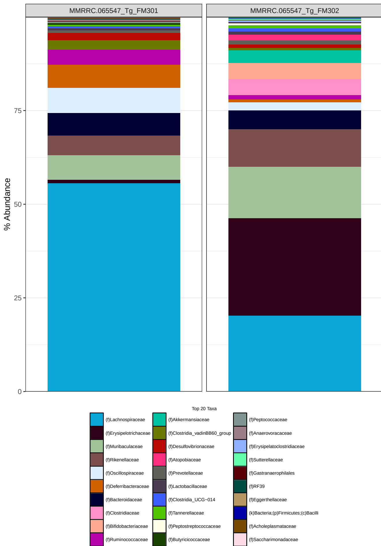
Figure 29: Family level abundances-FILTERED: 4 family level taxa removed
